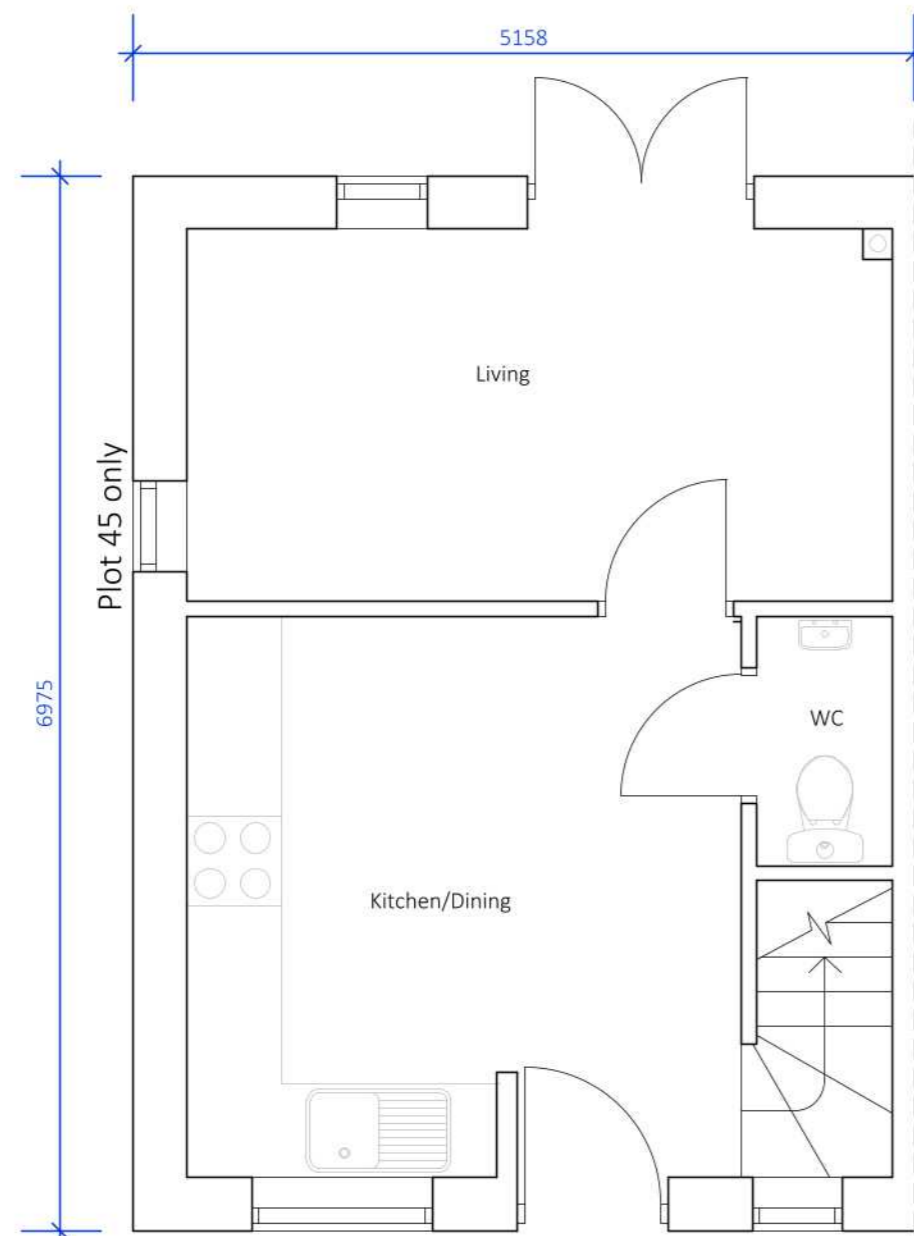
GROUND FLOOR PLAN GIA: 58sqm Plots 46 & 48 // Plots 45 & 47 handed
