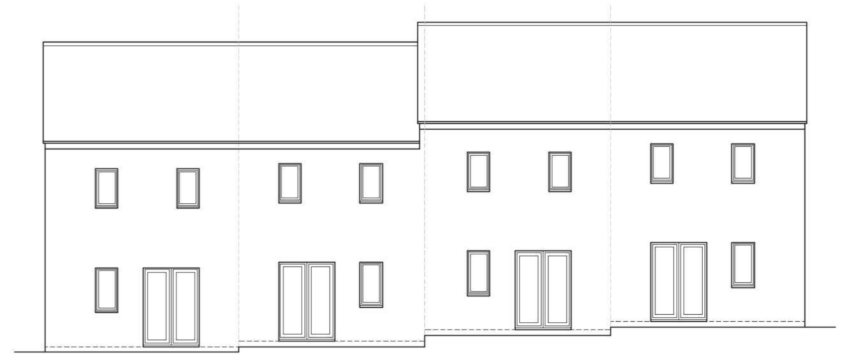
REAR ELEVATION [Plots 45 - 48]
