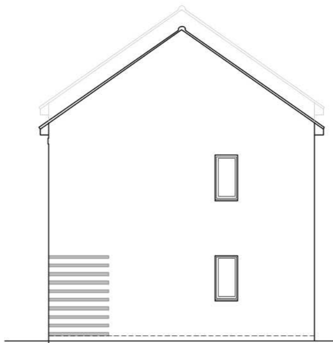
SIDE ELEVATION [Plot 45]
